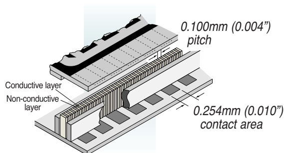
Typical ZEBRA® Connector interface between two contact areas; such as, PCB to LCD, or PCB to PCB.
